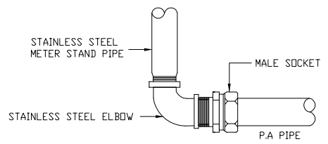
DETAIL 'A' POLY ALUMINIUM COMMUNICATION PIPE
