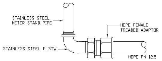
DETAIL 'A' HDPE PN 12.5 COMMUNICATION PIPE
