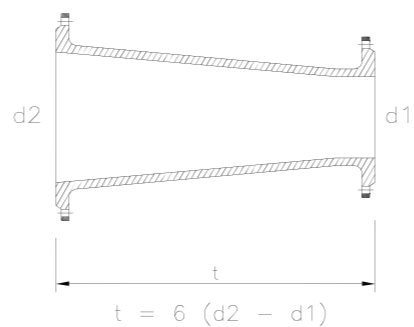
REDUCER DIMENSION
