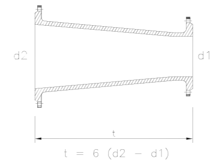
REDUCER DIMENSION
