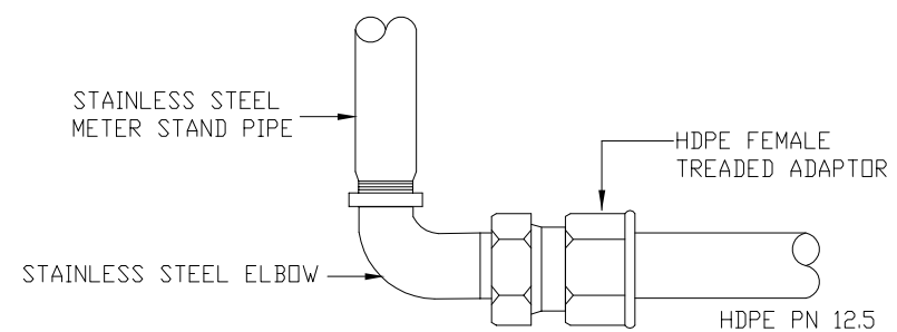
DETAIL 'A' HDPE PN 12.5 COMMUNICATION PIPE
