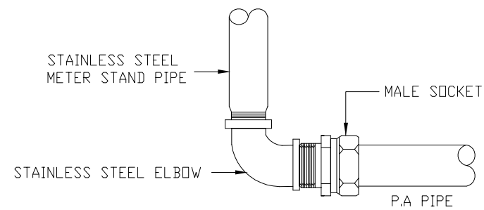
DETAIL 'A' POLY ALUMINIUM COMMUNICATION PIPE
