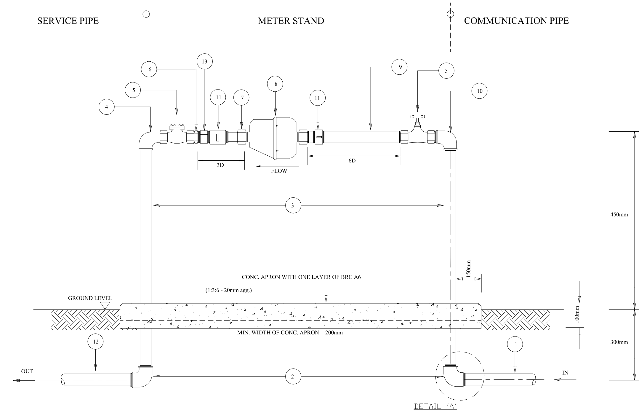
FRONT ELEVATION
