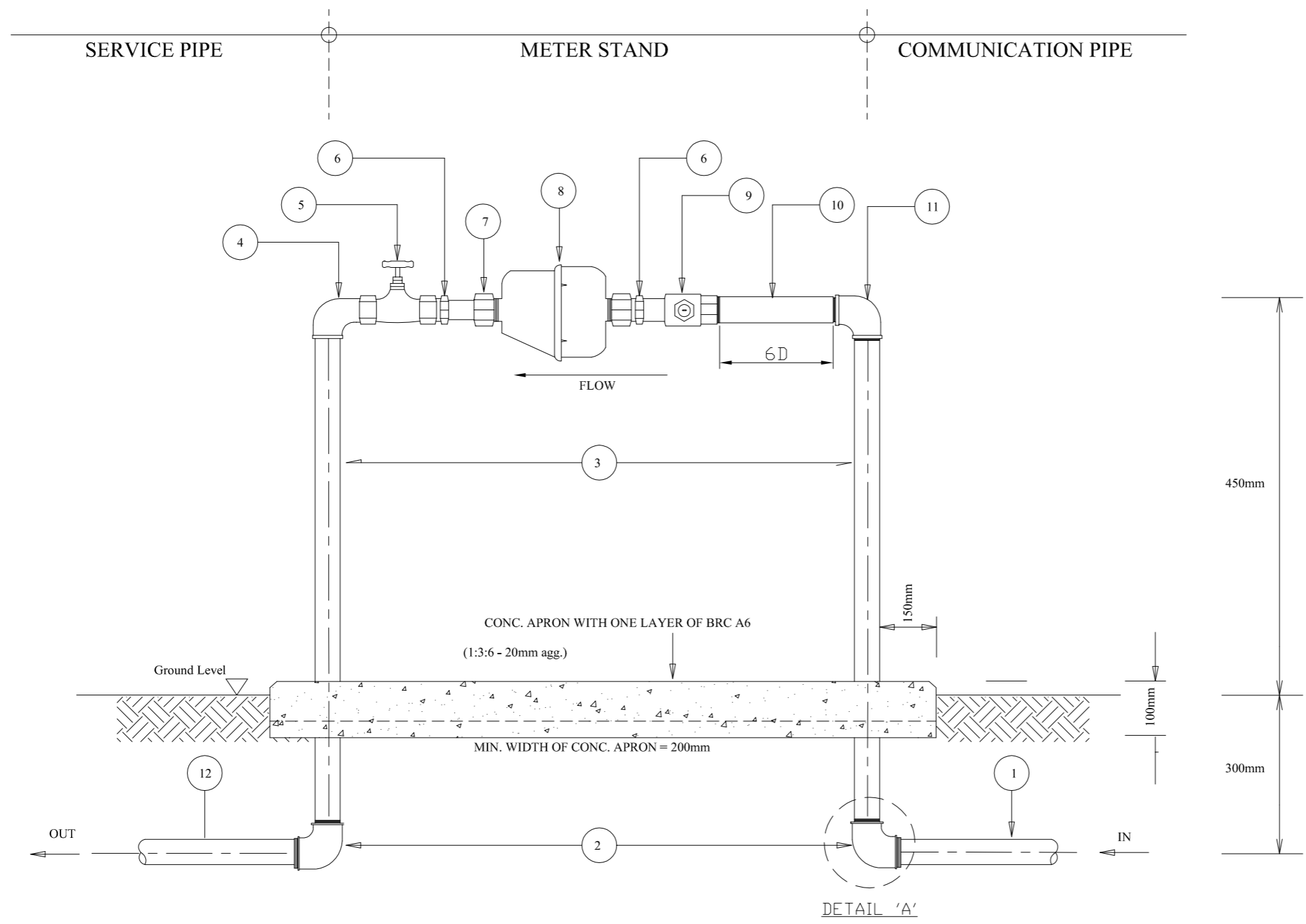
FRONT ELEVATION
