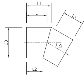
TYPE 1 GUSSETED BEND UP TO 30°
