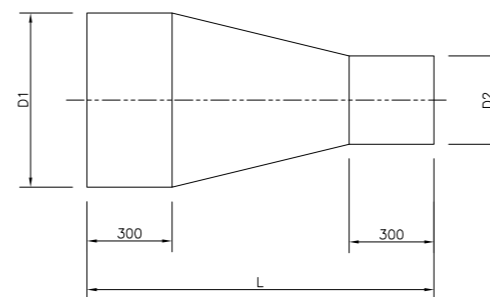
PLAIN ENDED CONCENTRIC TAPER
