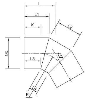
TYPE 2 GUSSETED BEND 31° TO 50°
