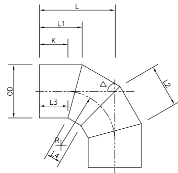
TYPE 3 GUSSETED BEND 61° TO 90° PLAIN ENDED BEND
