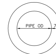
PUDDLE FLANGE DETAIL (THICKNESS = 15)
