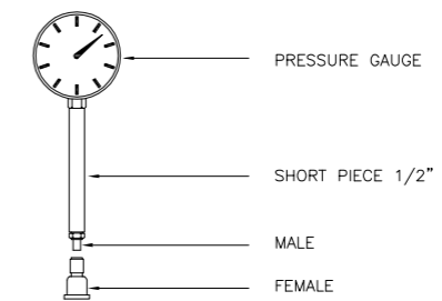
DETAIL OF DETACHABLE PRESSURE GAUGE
