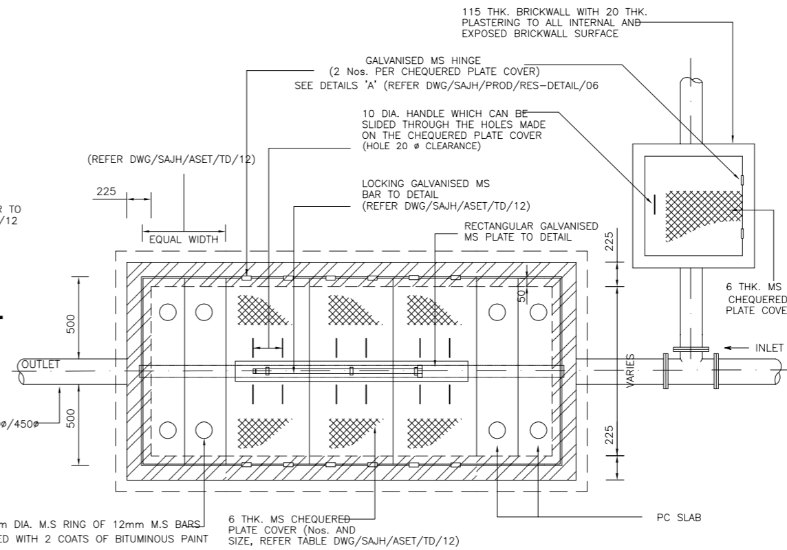
P.C. SLAB & CHEQUERED PLATE COVER
