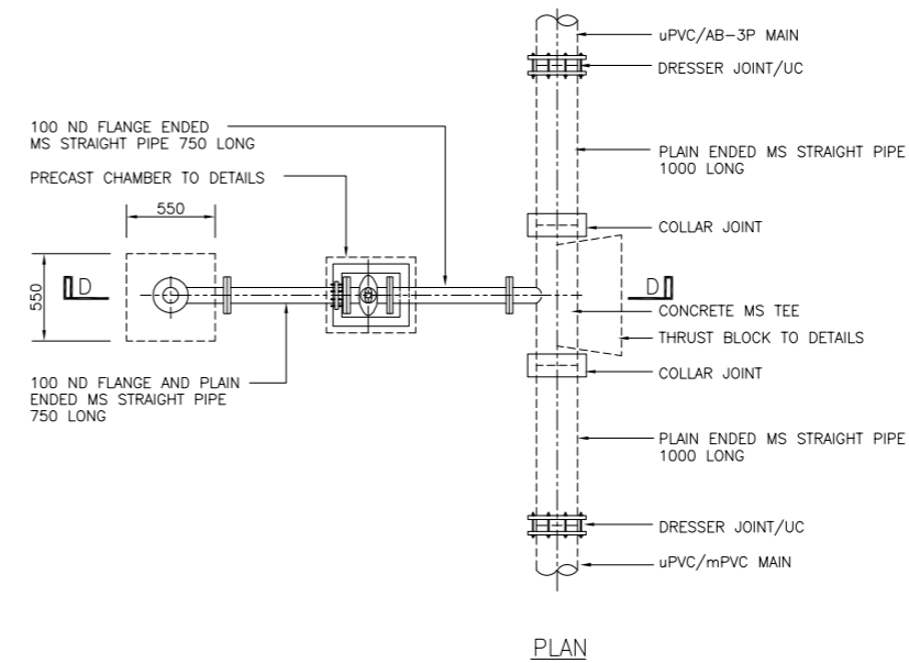
FIRE HYDRANT PRECAST CHAMBER WITH uPVC/mPVC PIPE ARRANGEMENT
