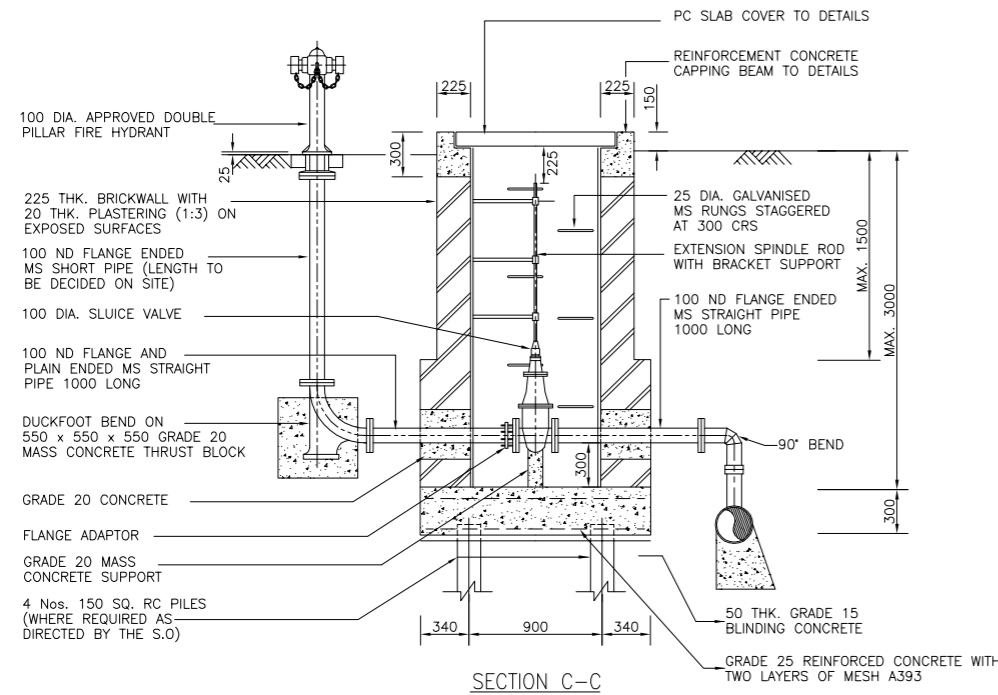
SECTION C-C
