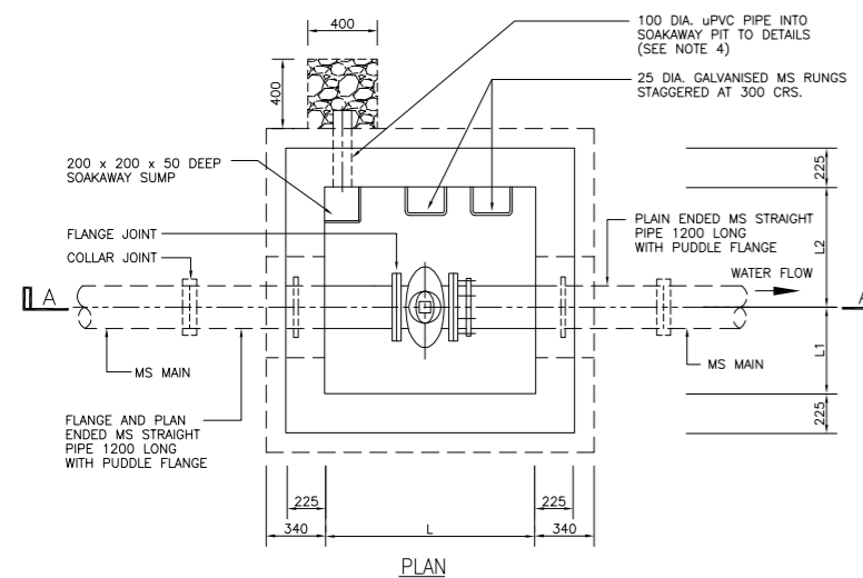
SLUIKE VALVE BRICKWALL CHAMBER WITH MS PIPE ARRANGEMENT
