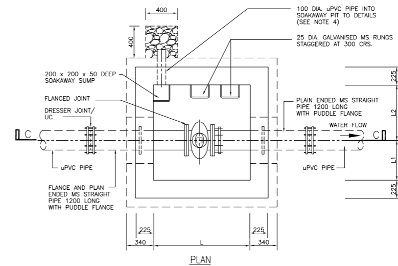
SLUIKE VALVE BRICKWALL CHAMBER WITH uPVC & mPVC PIPE ARRANGEMENT
