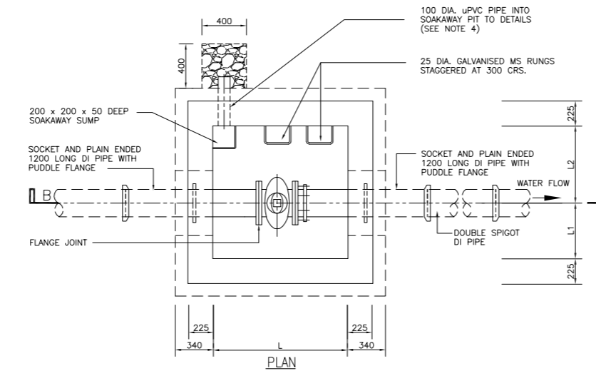
SLUIKE VALVE BRICKWALL CHAMBER WITH DI PIPE ARRANGEMENT (TYPE A)
