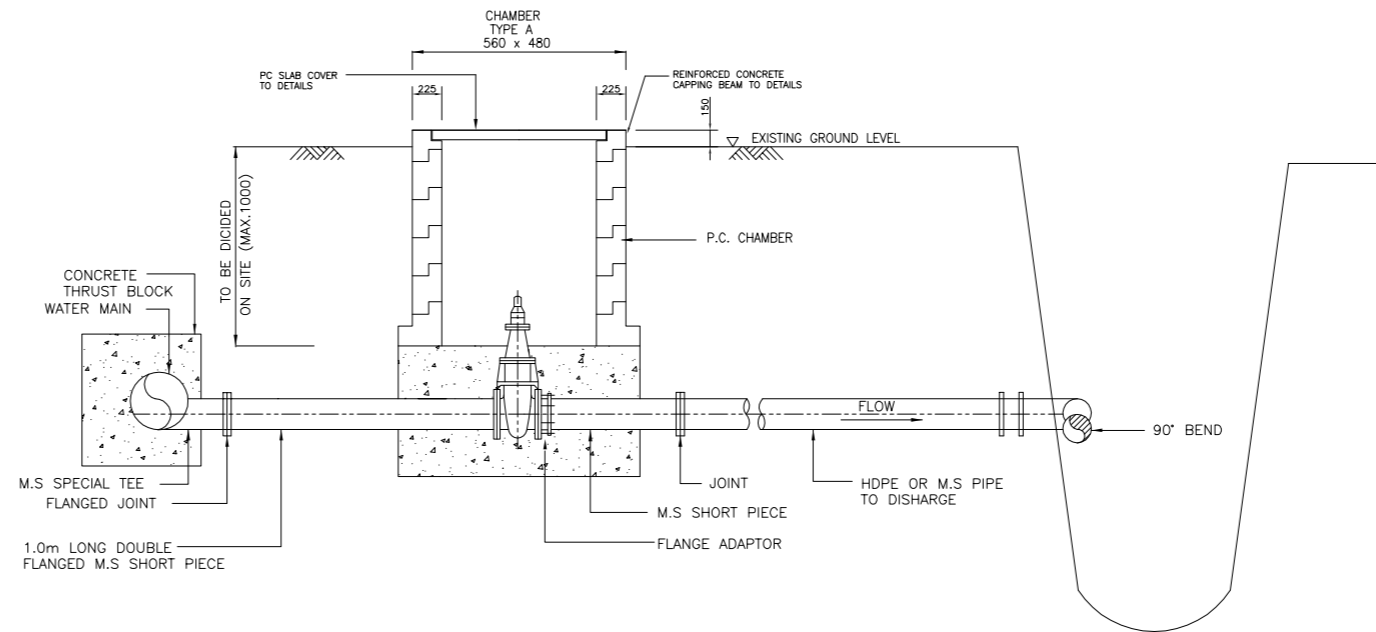
PC CHAMBER FOR SCOUR VALVE DEPTH LESS 1m
