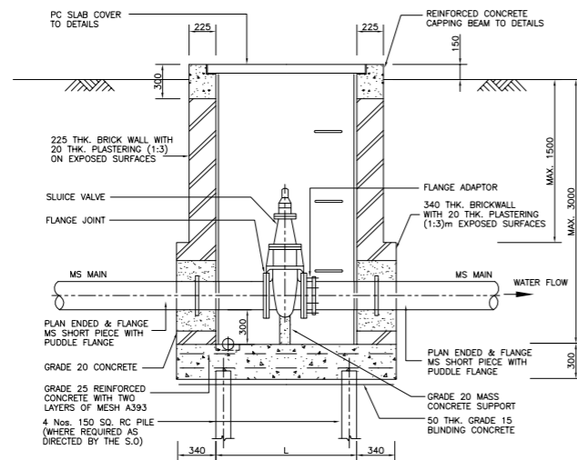
CHAMBER FOR SLUICE VALVE (FOR PIPE DEPTH 1m TO 1.5m)
