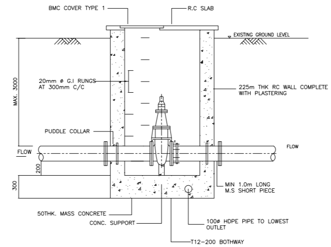
PC CHAMBER FOR SLUICE VALVE AND SCOUR VALVE (PIPE SIZE MORE THAN 600mm AND DEPTH MORE THAN 1.5m)
