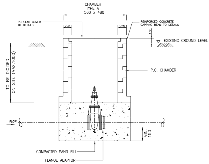
PC CHAMBER FOR SLUICE VALVE (DEPTH LESS THAN 1.0m)
